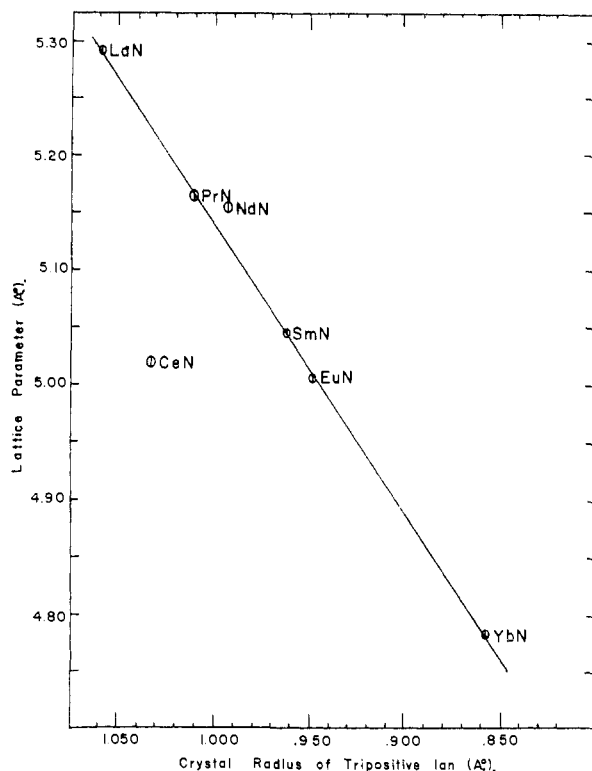
Fig. 1.—Comparison of the lattice properties of rare earth nitrides.
