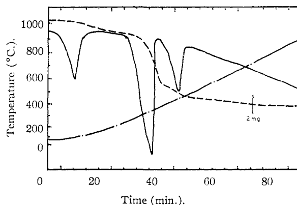
Fig. 2.—DTATGA curve of hydrolyzed SmN ( \text{Sm}(\text{OH})_3 ).
